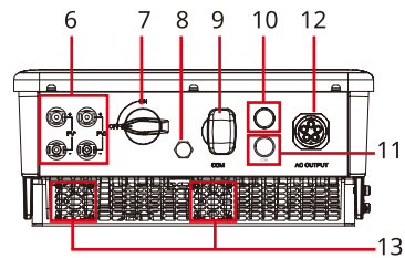
GW8K-DT, GW10KT-DT
